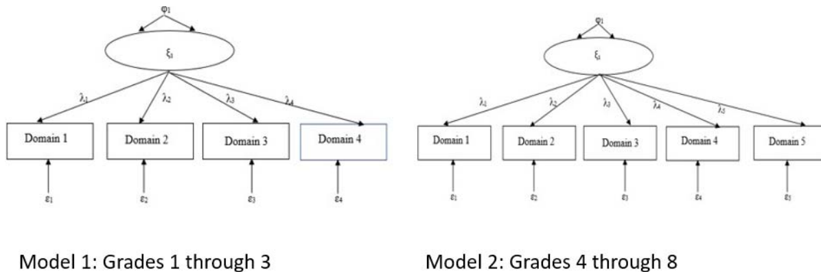
Figure 4: Confirmatory Factor Analyses (CFA) in Star Reading Spanish
