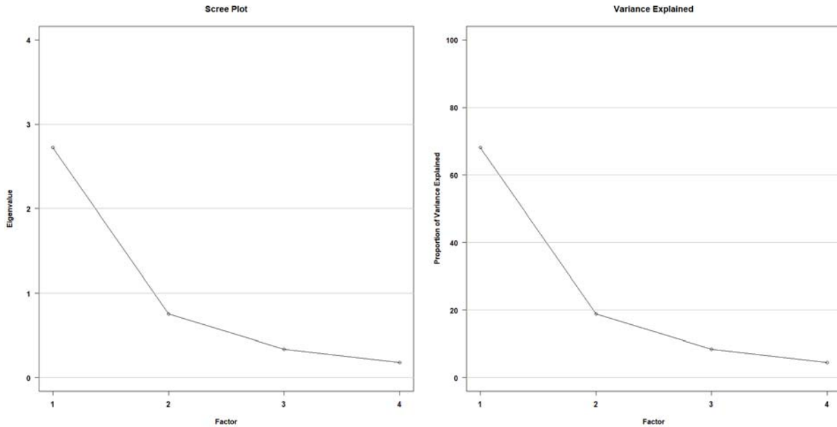
Figure 3: Scree Plot and Variance Explained by Factor Plot from the Grades 4 through 8 Exploratory Factor Analysis in Star Reading Spanish
